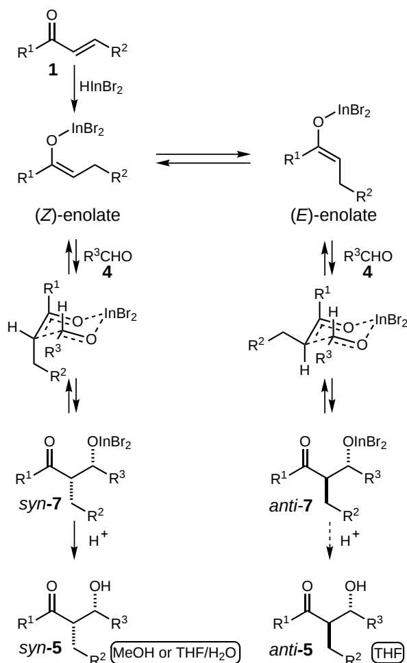
Scheme 1. Plausible reaction path.
